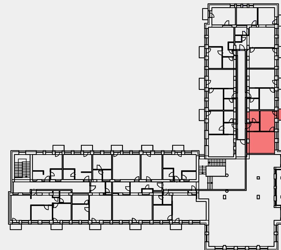
schéma pôdorysu 3. NP. / scheme of the 3. floor
